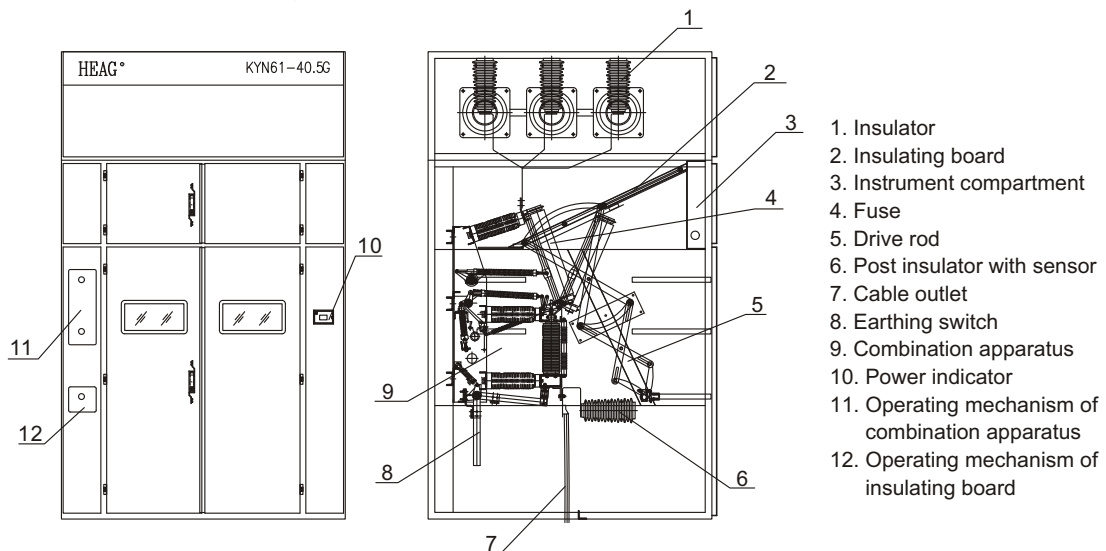
Diagram 2 FZR21-40.5 Into cubicle switchgear (KYN61) internal structure chart
