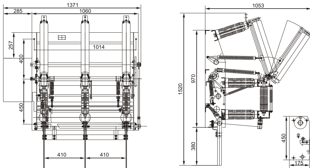
Diagram 1 FZR21-40.5/50-20 Outline dimension
